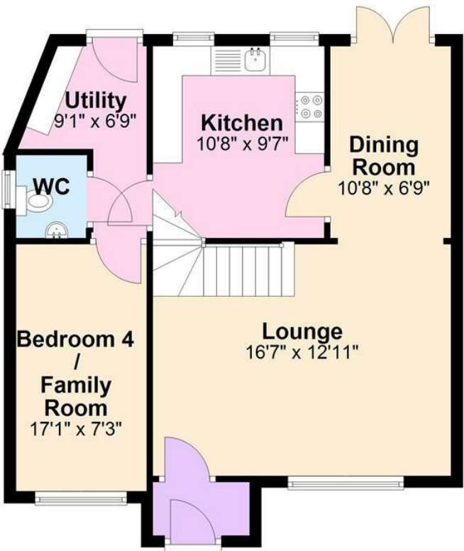
Ground Floor Approx. 586.1 sq. feet
